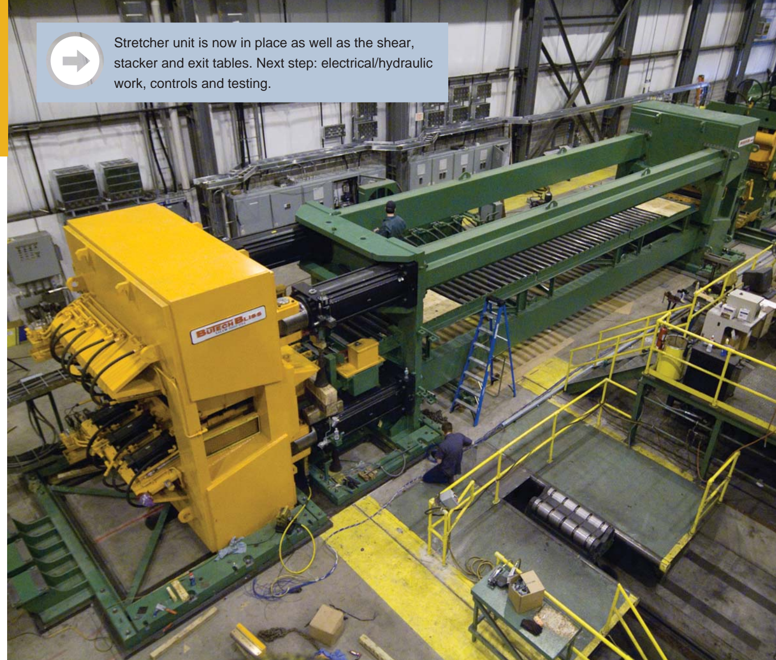
STRETCHER LEVELER
